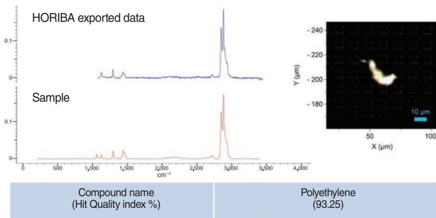
Supplementary Fig. 1. Examples of microphotographs and results of the Raman analysis of major microplastic types.
